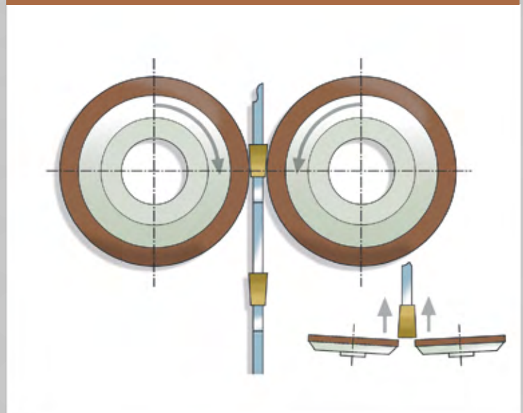
Side grinding
